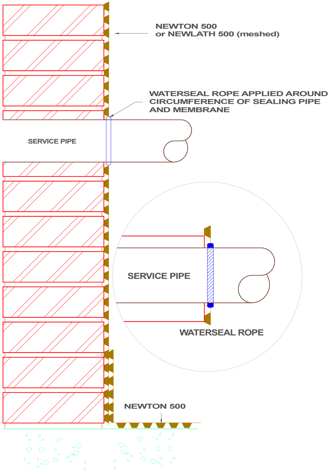
NEWTON SYSTEM 500 DETAIL AROUND SERVICE PIPE.
